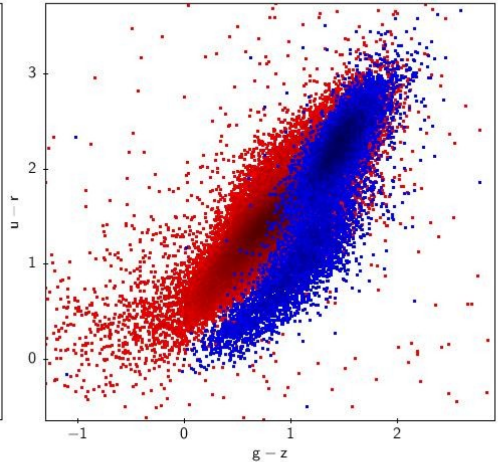
(u - r) vs. (g - z) color-color diagram for emission line objects in SDSS legacy survey
