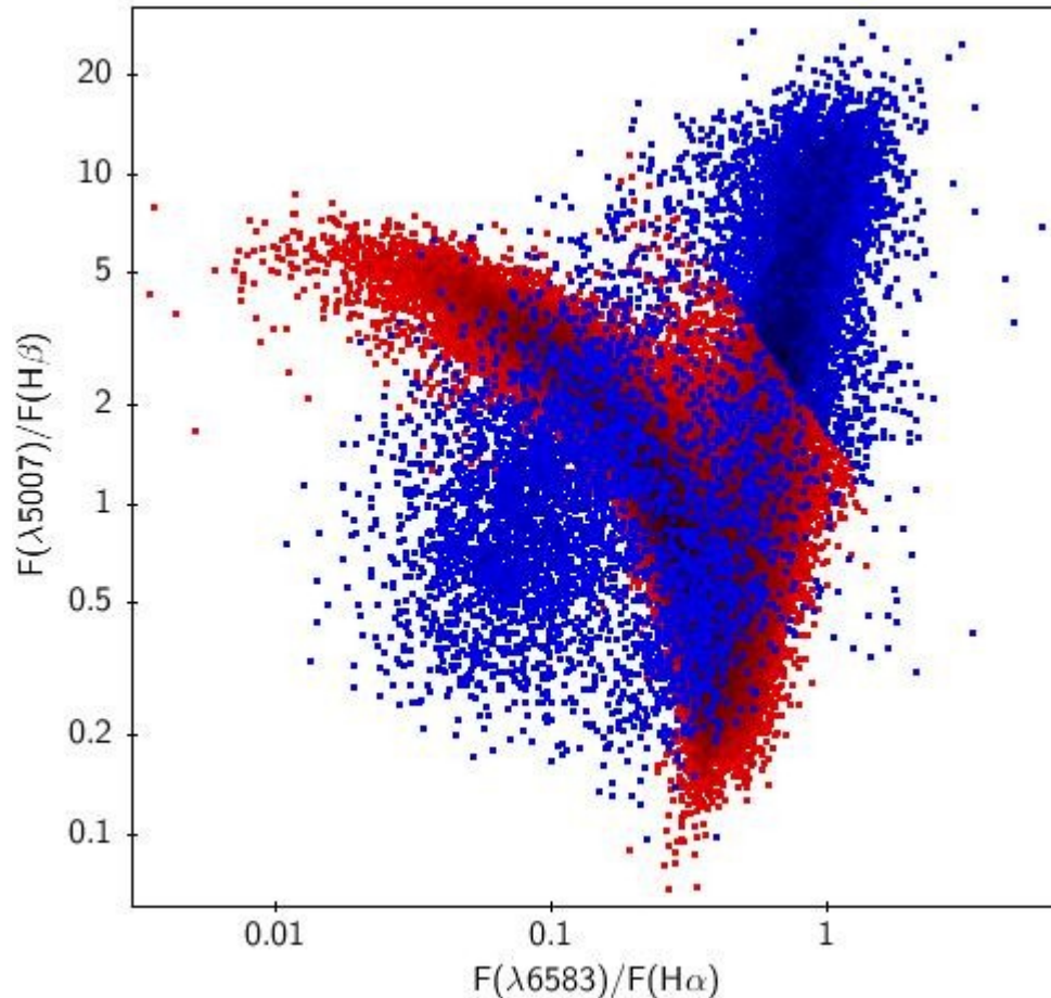
Classic BPT diagram, but for objects with both broad and narrow lines
